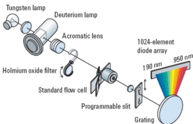
Diode array detector
