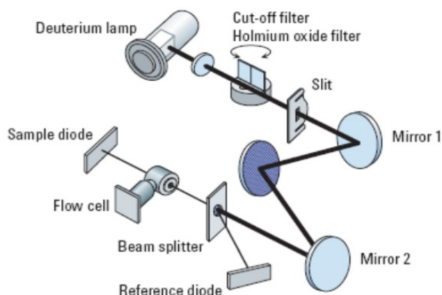
Single wavelength detector
